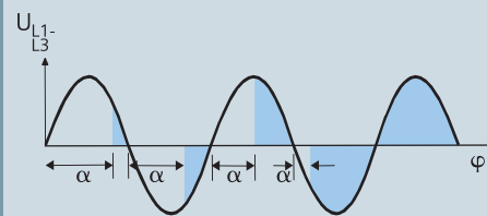
\alpha = Phase control angle
